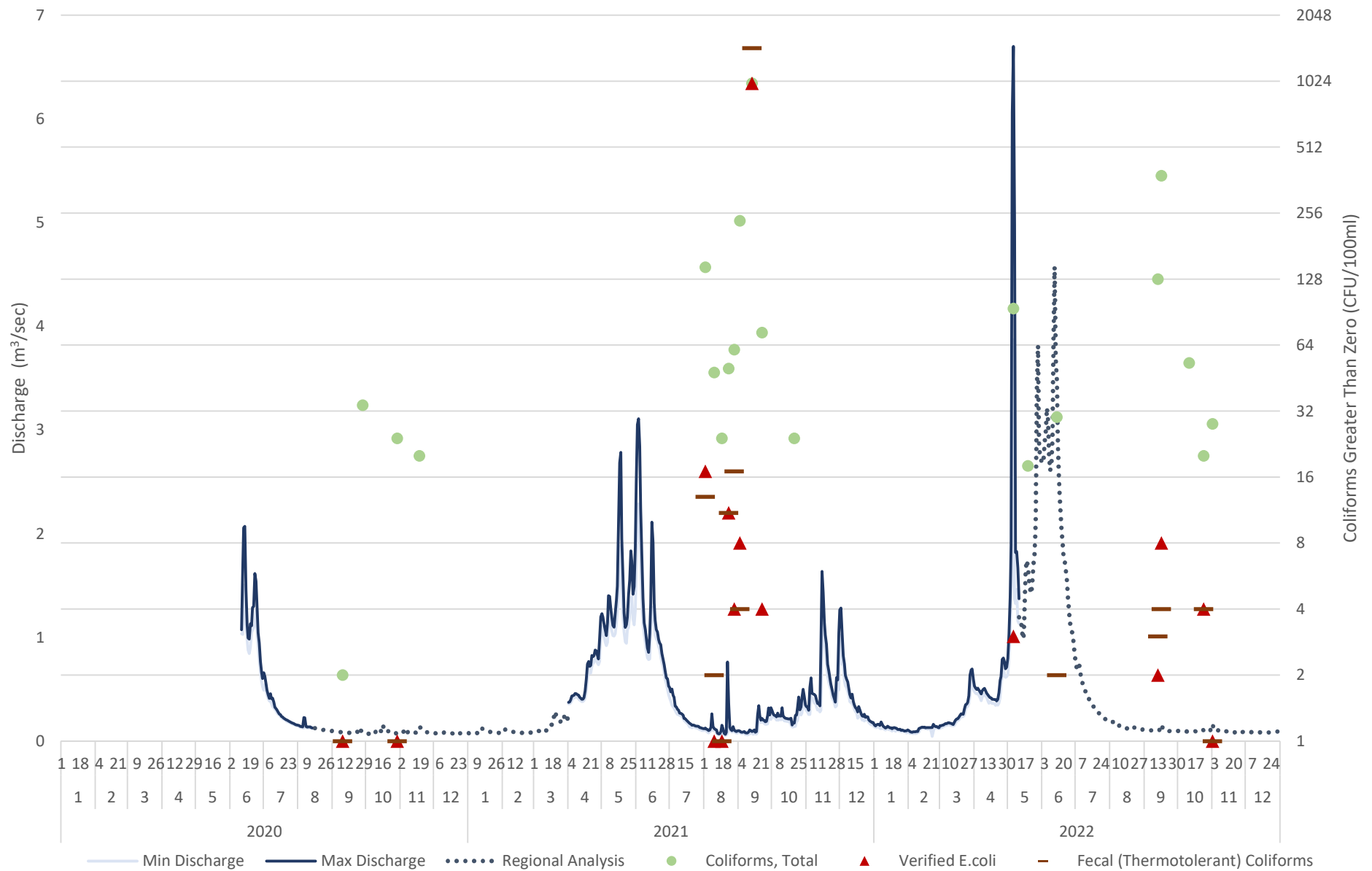
Trozzo Creek - Coliforms (Greater Than Zero) - Log Scale
